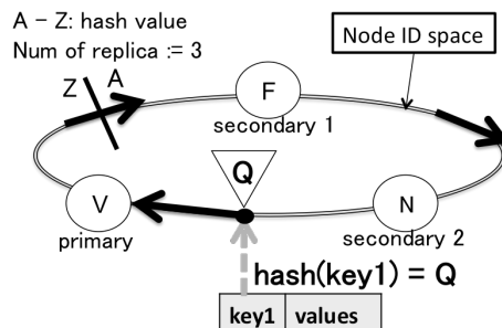
図 1 Consistent hashing Fig. 1 Consistent hashing
