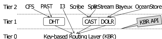
図 1 Key-based routing (KBR) (論文 19) の Figure 1) Fig. 1 Key-based routing (KBR) (Figure 1 from Dabek et al. 19) )
